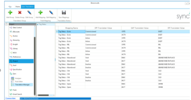
TRANSFORMATION RULE CONFIGURATION INTERFACE
